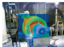
Fusion alpha
